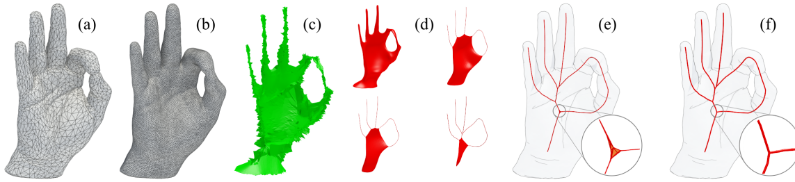
Figure 2: An overview of our skeletonization algorithm. The input mesh (a) is first remeshed (b) to obtain better-quality Voronoi poles, from which a medial skeleton is computed (c) to constrain our construction of a medially centered skeleton. The algorithm performs iterative mesh contraction to generate a series of meso-skeletons in intermediate steps (d). Note that mesh connectivity is simplified throughout the contraction process. The last iteration produces a thin skeletal structure (e) which is finally converted into a curve skeleton (f) via edge collapse. The inserts in (e) and (f) show close-ups at the center of the palm.
